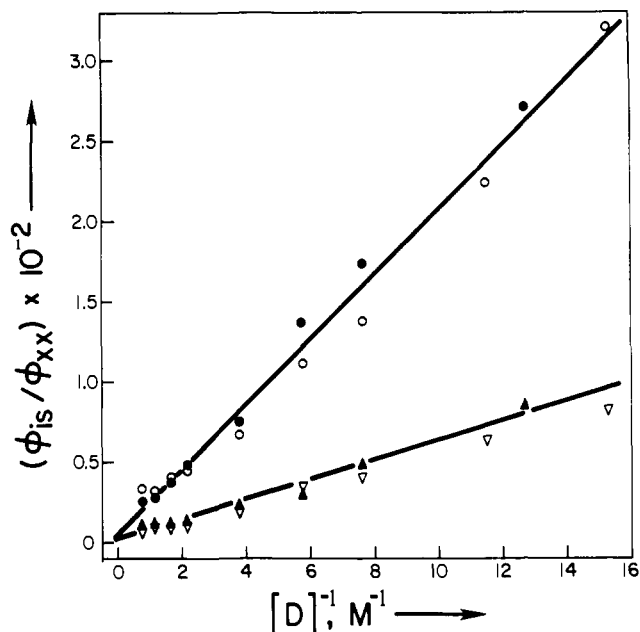
Figure 2. Diene concentration dependence of diene isomerization quantum yields in degassed solutions: (O) \phi_{tt \rightarrow cc} , (▽) \phi_{tt \rightarrow tc} , (●) \phi_{tt \rightarrow cc} with 10^{-2} M c-St , (▲) \phi_{tt \rightarrow tc} with 10^{-2} M c-St .
