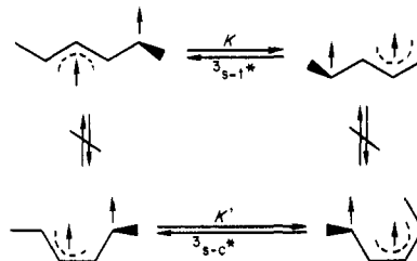
Scheme I. Dynamic Behavior of 2,4-Hexadiene Triplets
