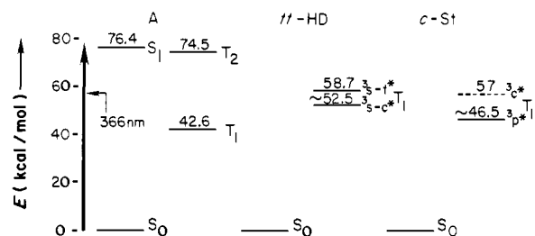
Figure 1. Donor-acceptor-state diagram.
