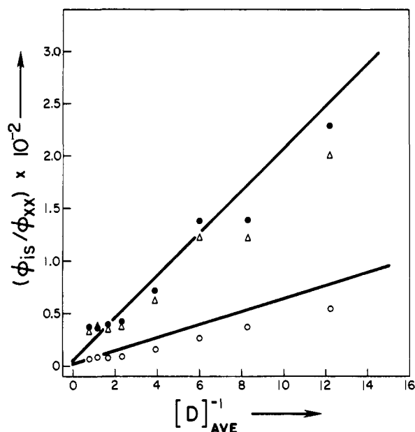
Figure 3. Diene concentration dependence of diene isomerization quantum yields in air-saturated solutions: (●) \phi_{tt \rightarrow cc} and (○) \phi_{tt \rightarrow cc} by using eq 16 for \phi_{is} ; (▲) \phi_{tt \rightarrow cc} by using eq 14 for \phi_{is} ; lines are taken from Figure 2.
